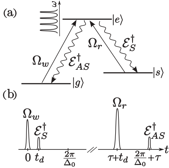
FIG. 1. (a) Basic level scheme and (b) pulse sequence for the creation of correlated Stokes–anti-Stokes pairs via spontaneous Raman emission. All atoms start in g . The inhomogeneously broadened optical transition is shaped into an atomic frequency comb. A resonant write pulse \Omega_w excites the g - e transition, making possible the spontaneous emission of a Stokes photon. The detection of a Stokes photon (at time t_d ) is uniquely correlated with the creation of a single collective atomic excitation corresponding to one excitation in S delocalized over all the atoms. This collective excitation can be mapped very efficiently into an anti-Stokes photon using a resonant read pulse \Omega_r (at time \tau + t_d ) and benefiting from the echo-photon-type re-emission (at time 2\pi/\Delta + \tau ) inherent to inhomogeneous transition shaped into a frequency comb.
